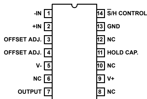
HA-2420 (CERDIP) TOP VIEW
