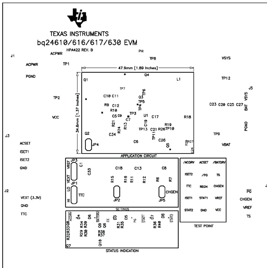
Figure 8. Top Silkscreen
