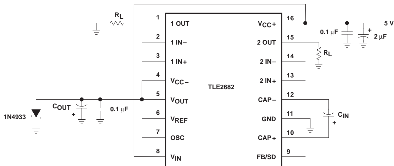
Figure 6. Bias-Current Test Circuit
