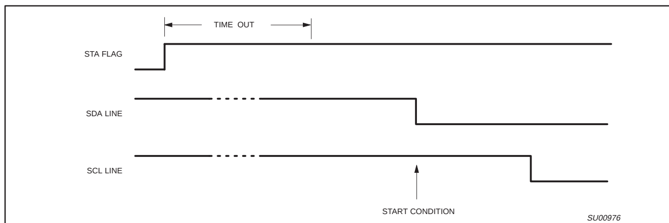
Figure 7. Forced access to a busy I 2 C-bus
