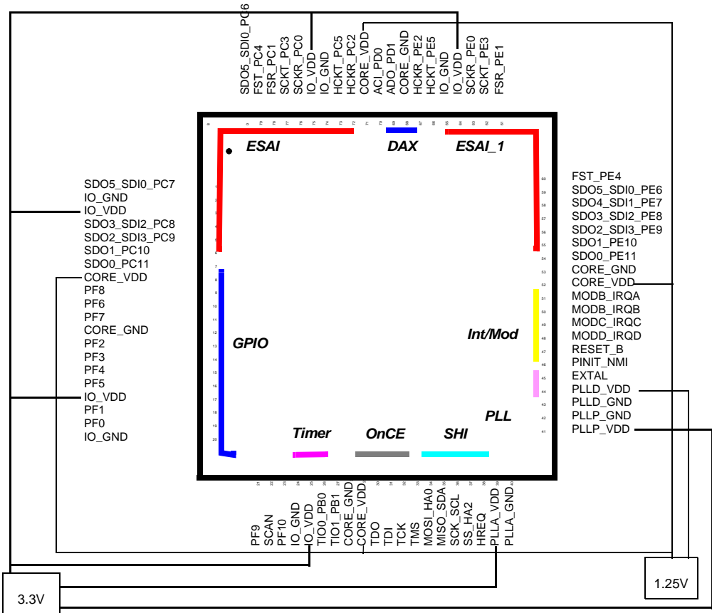
Figure 3. VDD Connections
