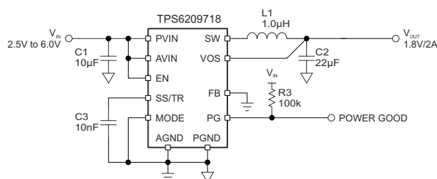
1.8-V Output, PWM/PSM Mode Application
