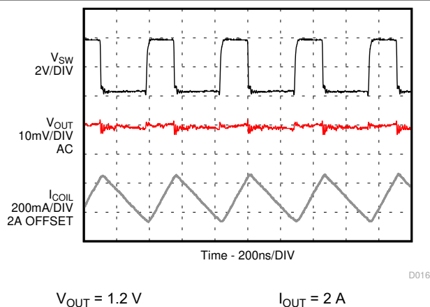
Figure 9-15. Output Ripple, PWM Operation (2.0 MHz)
