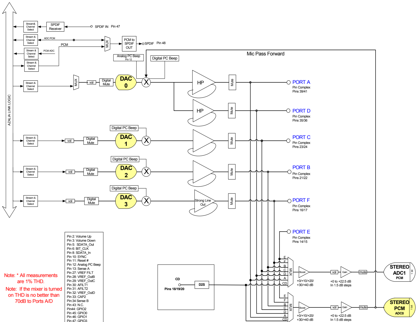
Figure 1. Functional Block Diagram - 92HD202
