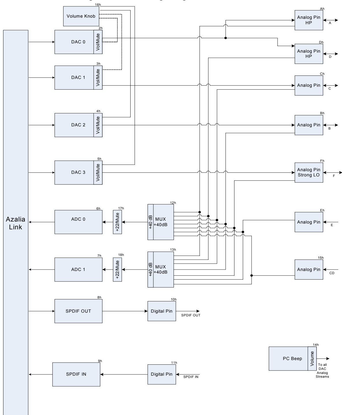
Figure 3. 92HD202 Widget Diagrams
