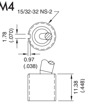
15/32" threaded
