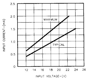
FIGURE 4. INPUT CHARACTERISTICS - SG2002
