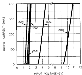
FIGURE 2. OUTPUT CURRENT VS. INPUT VOLTAGE
