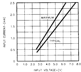
FIGURE 5. INPUT CHARACTERISTICS - SG2003
