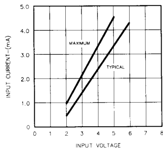
FIGURE 7. INPUT CHARACTERISTICS - SG2005
