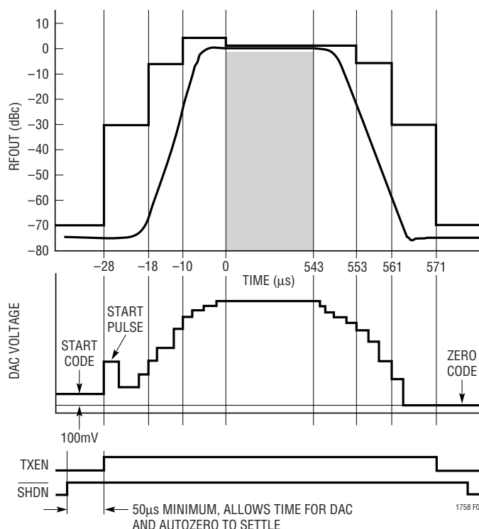
Figure 1. LTC1758 Ramp Timing
