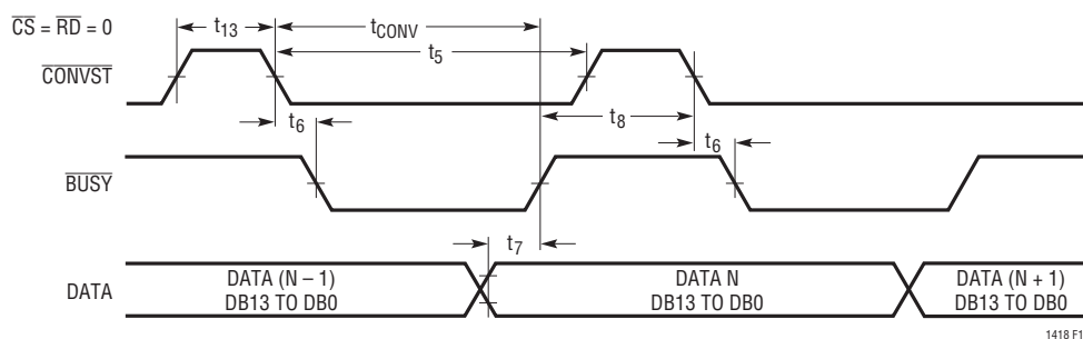
Figure 16. Mode 1b. \overline{\text{CONVST}} Starts a Conversion. Data Outputs Always Enabled ( \overline{\text{CONVST}} = \text{[Pulse]} \text{ )}
