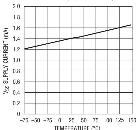
V_{SS} Supply Current vs Temperature (Bipolar Mode)
