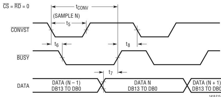
Figure 15. Mode 1a. \overline{\text{CONVST}} Starts a Conversion. Data Outputs Always Enabled ( \overline{\text{CONVST}} = \text{[Pulse]} \text{ )}
