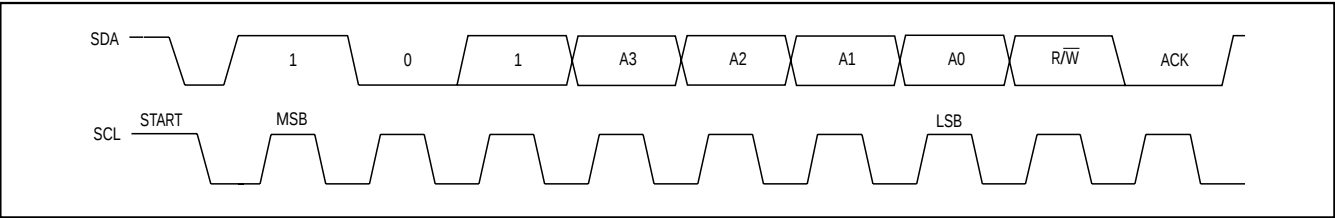
Figure 6. Slave Address
