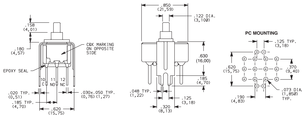
8421SD3V4GE 4PDT
