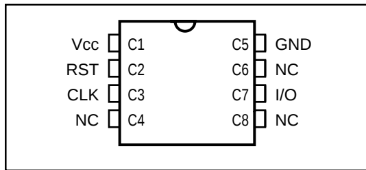
Figure 2. Pin Configuration
