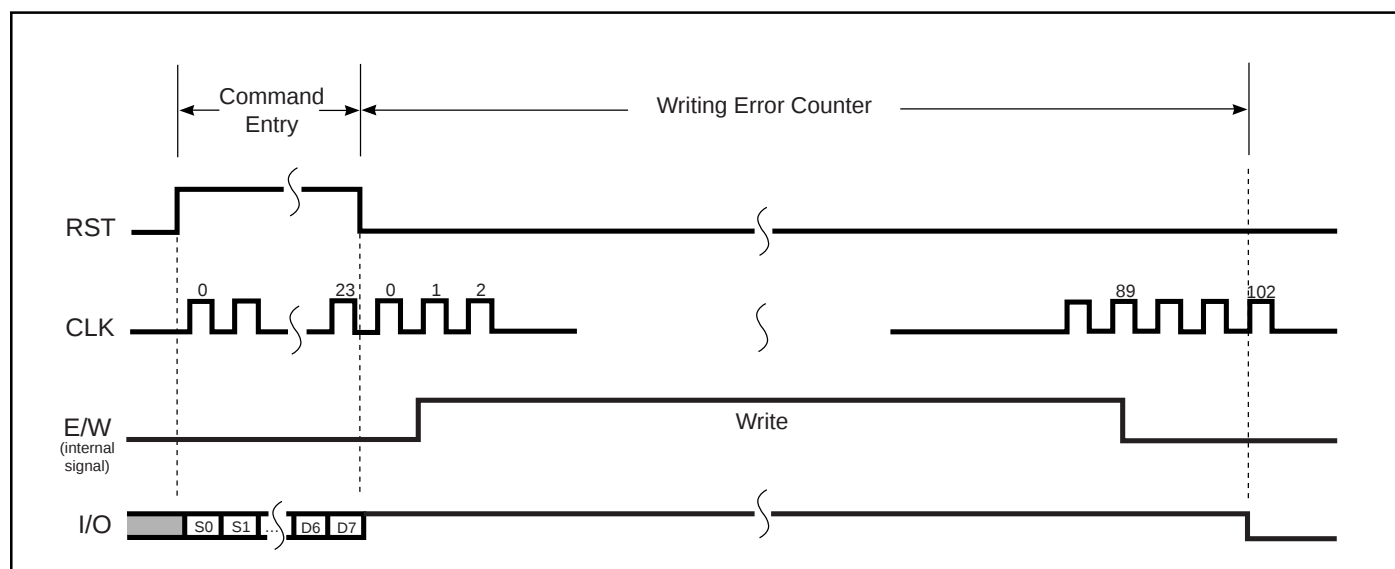
Figure 10. Writing Error Counter
