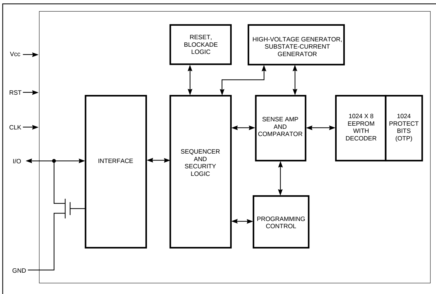
Figure 1. Block Diagram
