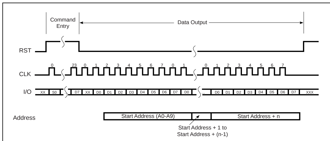
Figure 6. Read 8-bit Data
