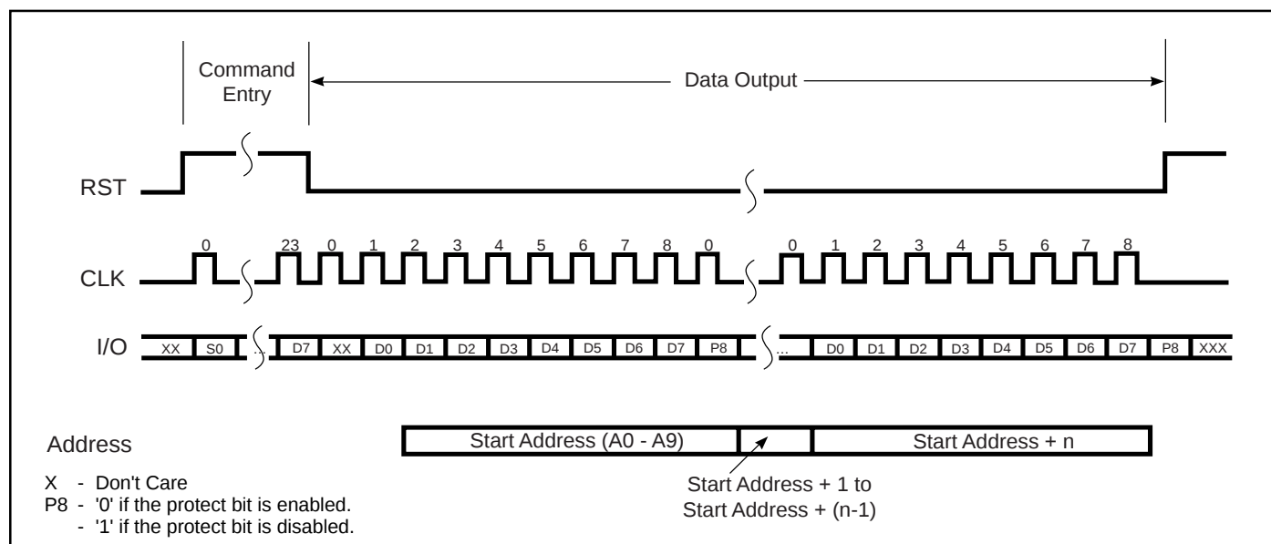
Figure 7. Read 9-bit Data with Protect Bit
