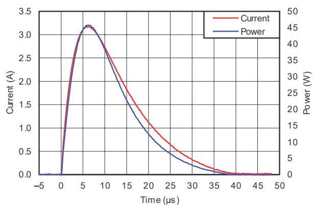
Figure 5-2. Surge Curve ( t_p = 8/20 \mu s ), Pin IO to GND
