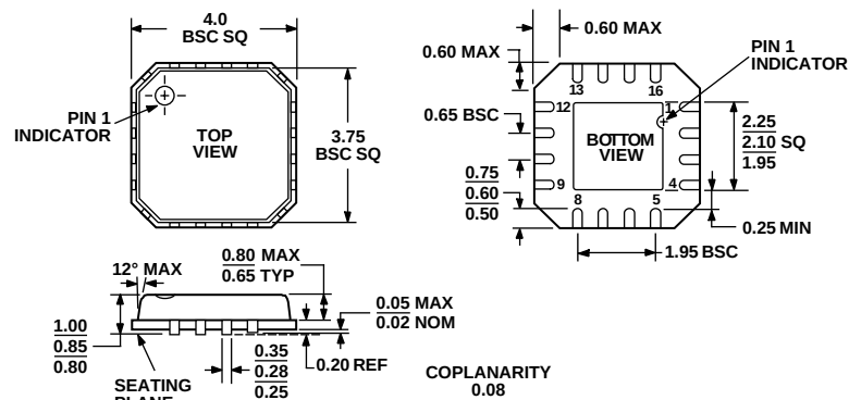
Figure 42. 16-Lead Lead Frame Chip Scale Package [LFCSP] (CP-16) Dimensions shown in millimeters
