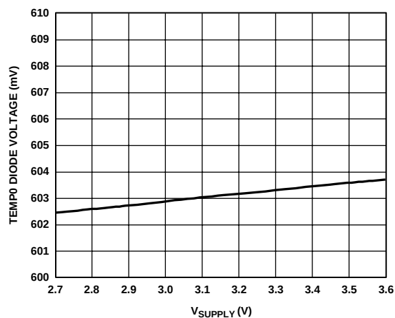
Figure 21. Temp0 Diode Voltage vs. V_{SUPPLY} (25°C)
