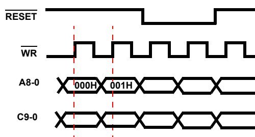
FIGURE 2. LATCHING C9-0 VALUES INTO ADDRESS A8-0 REGISTERS
