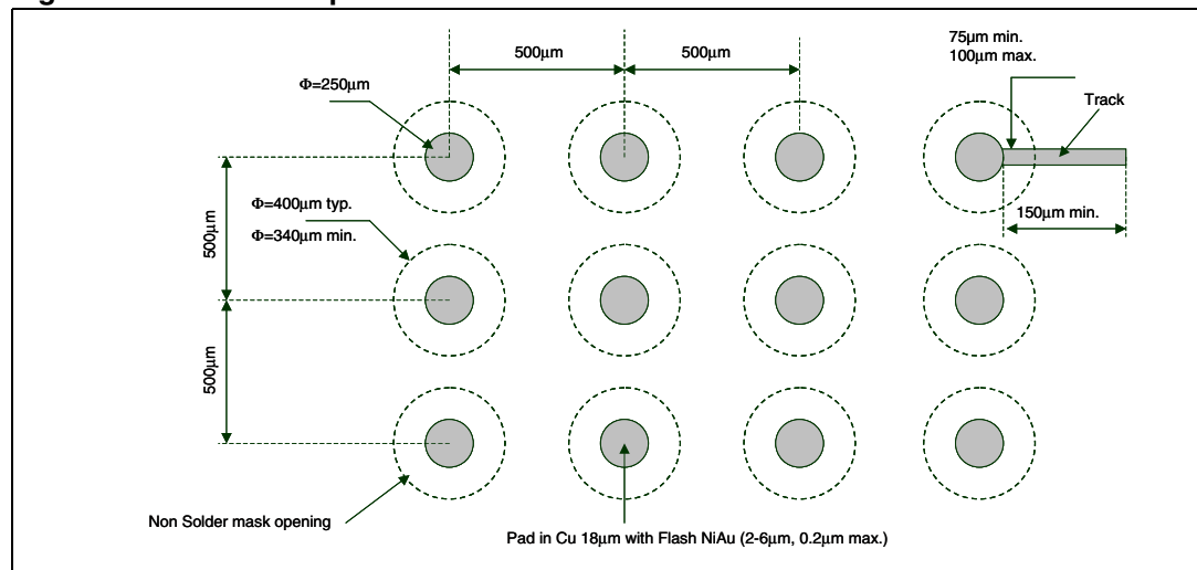
Figure 43. TS472 footprint recommendation
