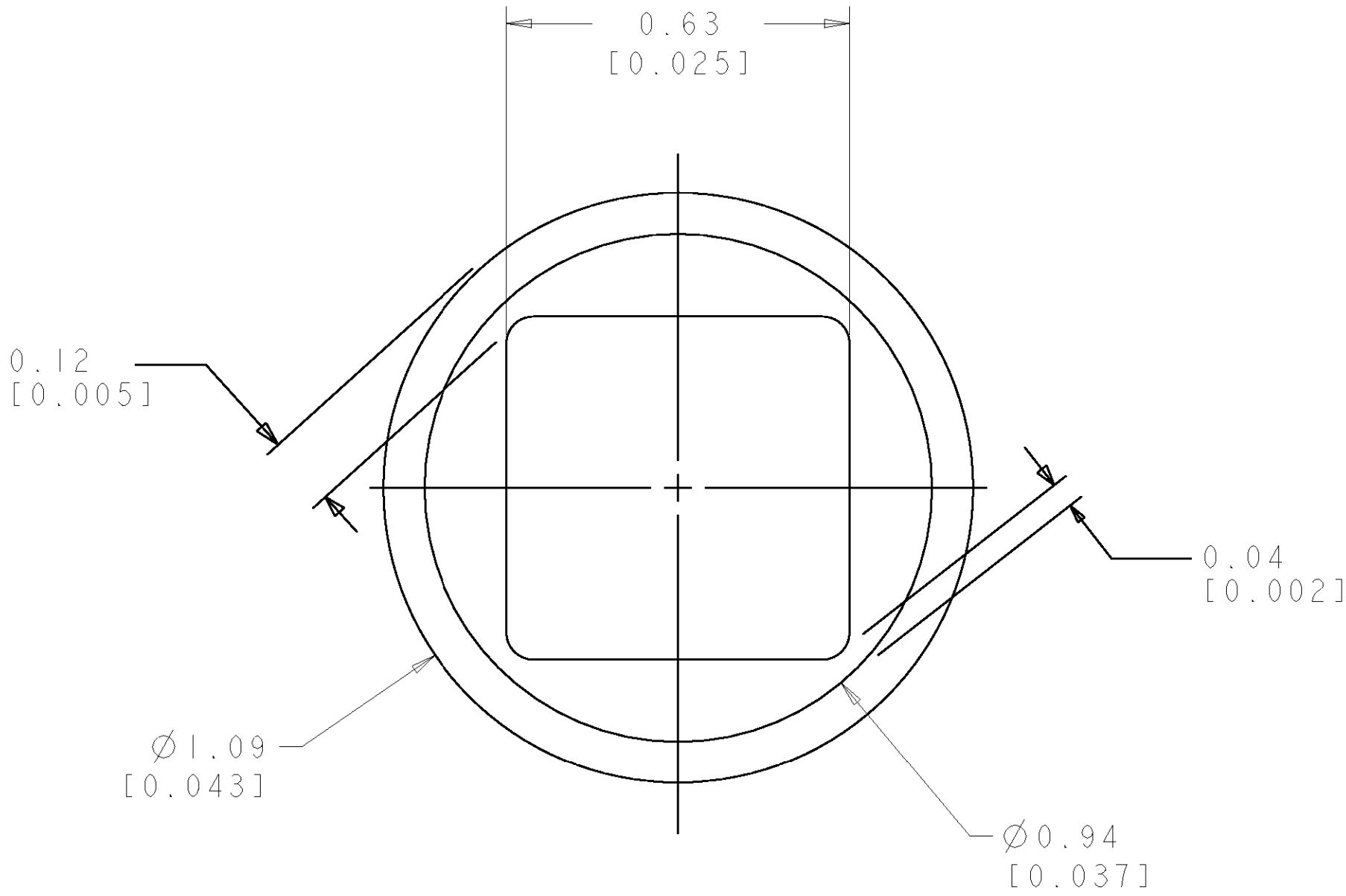
SOLDER TERMNIATION AREA SCALE 40:1 RECOMMENDED PRINTED CIRCUIT SOLDER HOLE FINISHED HOLE: Ø 1.02 [ .040 ] ± 0.08 [ .003 ] DRILLED HOLE: Ø 1.15 [ .0453 ] ± 0.013 [ .0005 ] COPPER PLATE: 0.025 [ .0010 ] MIN TIN PLATE: 0.008 [ .0003 ] MIN. (PER SURFACE)
