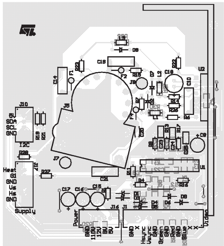
Figure 2. TDA9535/9536 - TDA9210 - Demonstration Board: Silk Screen and Trace (scale 1:1)
