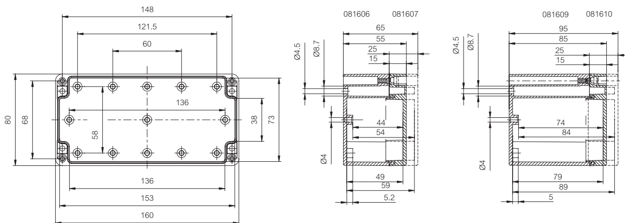
EURONORD PC/ABS 160x80x55-95
