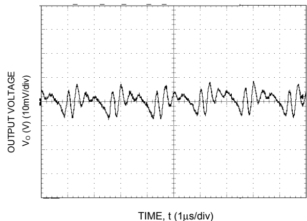
Figure 3. Typical output ripple and noise (C O =10μF ceramic, V IN = 12V, I o = I o,max ).
