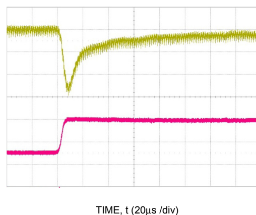
Figure 28 Transient Response to Dynamic Load Change from 50% to 100% at 12Vin, C_{out} = 2 \times 47\mu\text{F} , C_{Tune}=2200\text{pF} & R_{Tune}=267
