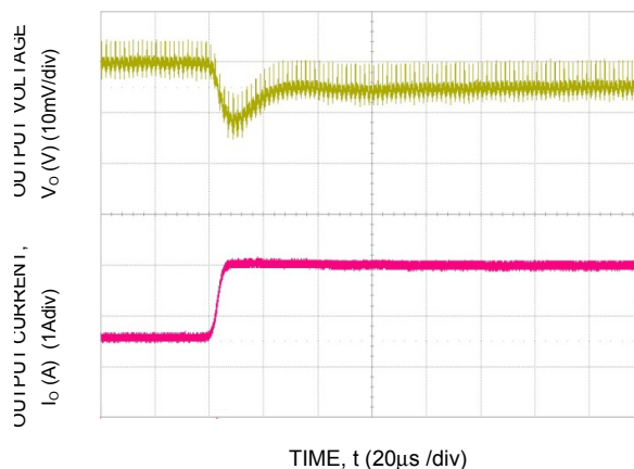
Figure 4. Transient Response to Dynamic Load Change from 50% to 100% at 12Vin, C out =1x47μF+2x330μF, C Tune =27nF, R Tune =180
