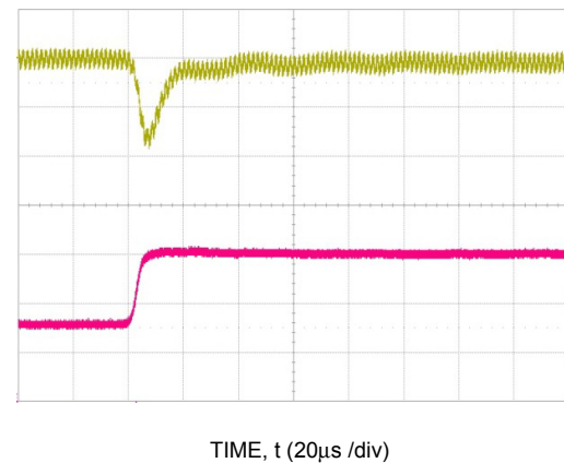
Figure 34. Transient Response to Dynamic Load Change from 50% to 100% at 12Vin, C_{out}=1x47\mu F , C_{Tune}=820pF & R_{Tune}=267
