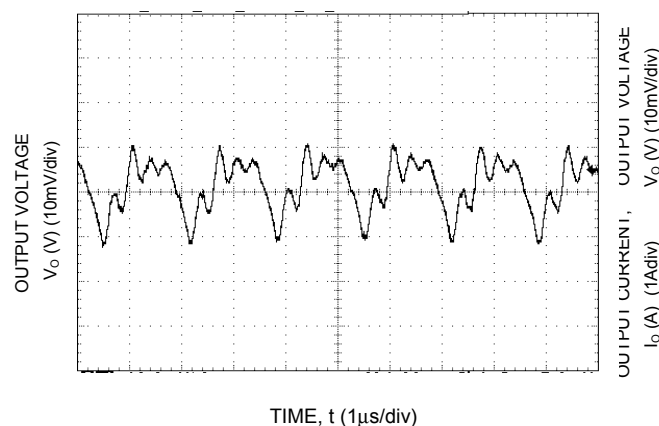
Figure 15. Typical output ripple and noise ( C_o=10\mu\text{F} ceramic, V_{IN} = 12\text{V} , I_o = I_{o,max} ).
