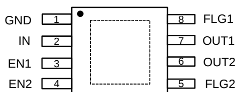
MSOP-8EP
