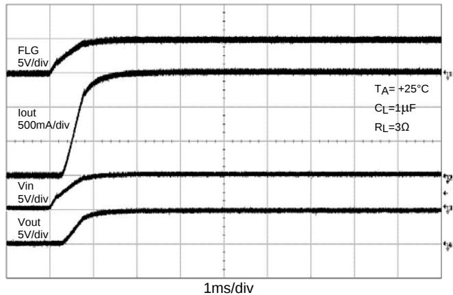
Device Enabled
