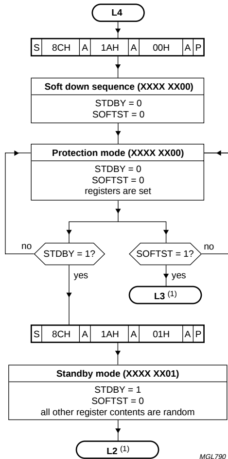
Fig.19 I 2 C-bus flow for protection and standby mode.
