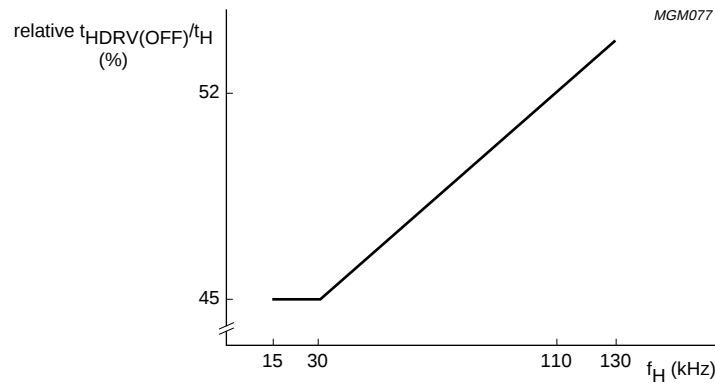
Fig.16 Relative t_{OFF} time of HDRV as a function of horizontal frequency.
