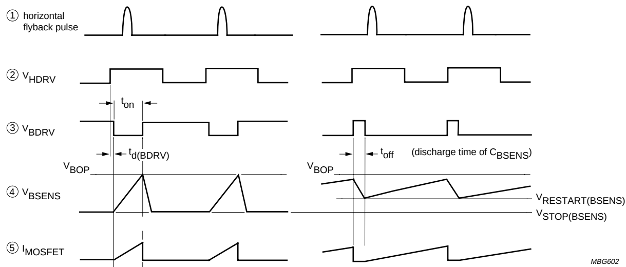
b. Waveforms for normal operation. c. Waveforms for fault condition.
