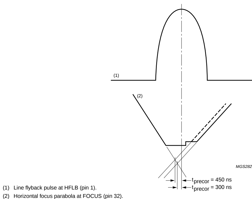
Fig.28 Definition of H-focus pre-correction.
