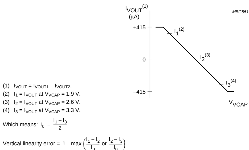
Fig.27 Definition of vertical linearity error.
