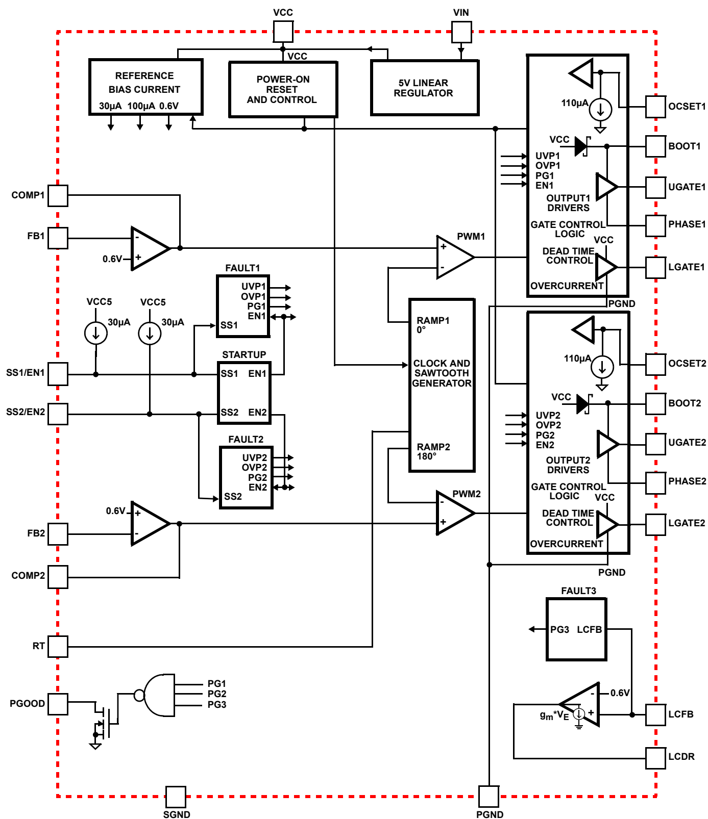
FIGURE 3. BLOCK DIAGRAM
