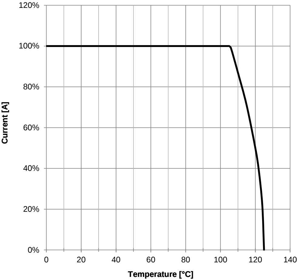
Derating Curve:
