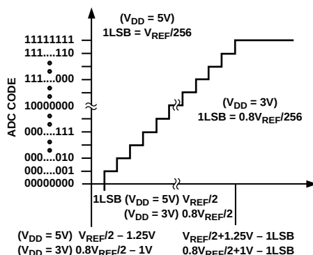
Figure 6. Transfer Characteristic
