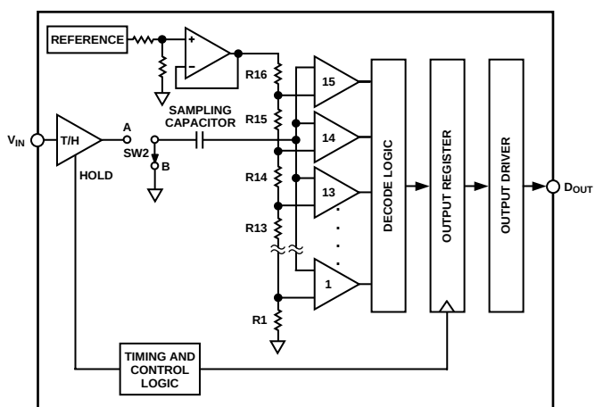
Figure 3. ADC Conversion Phase
