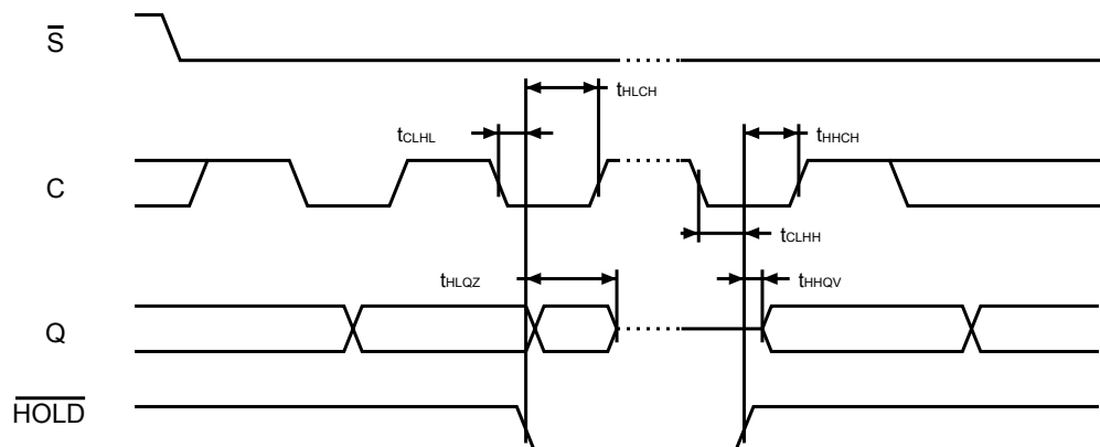
Figure 21. Hold timing
