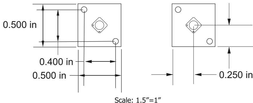
Figure 1. Mounting centers
