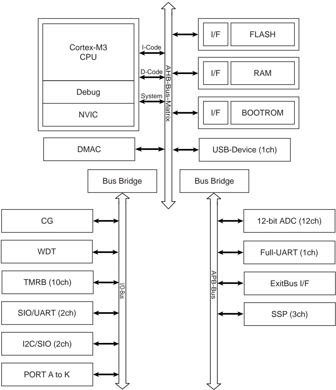
Figure 1-1 TMPM366FDXBG/FYXBG/FWXBGBlock Diagram
