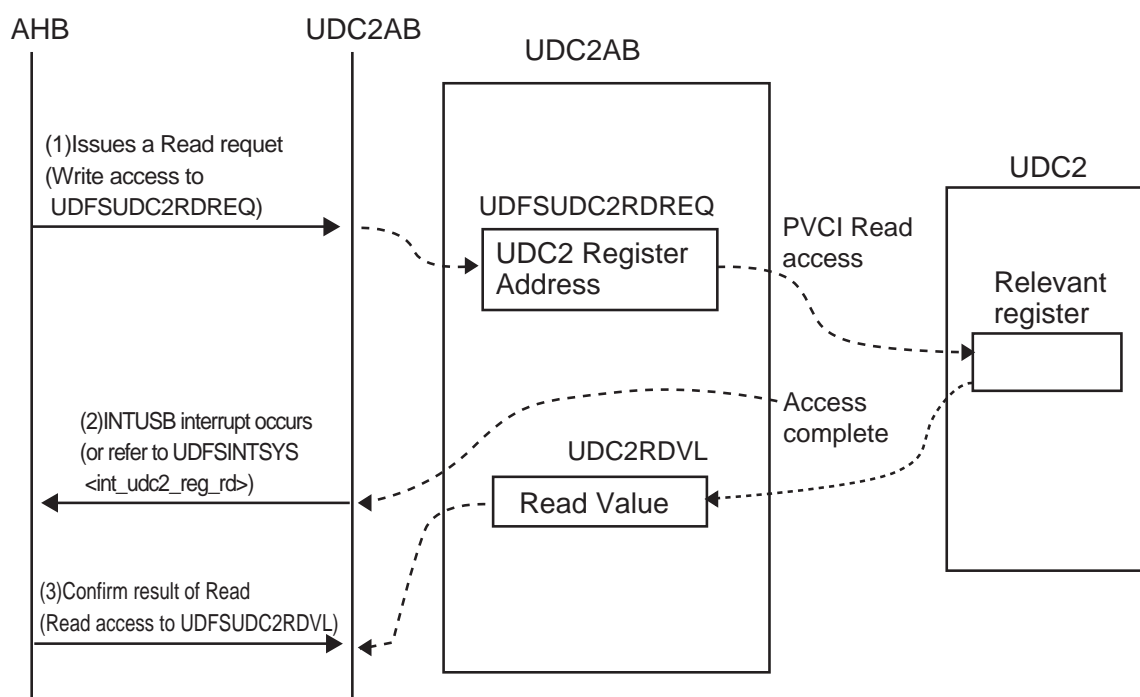
Figure 14-7 Read access flow for UDC2 register
