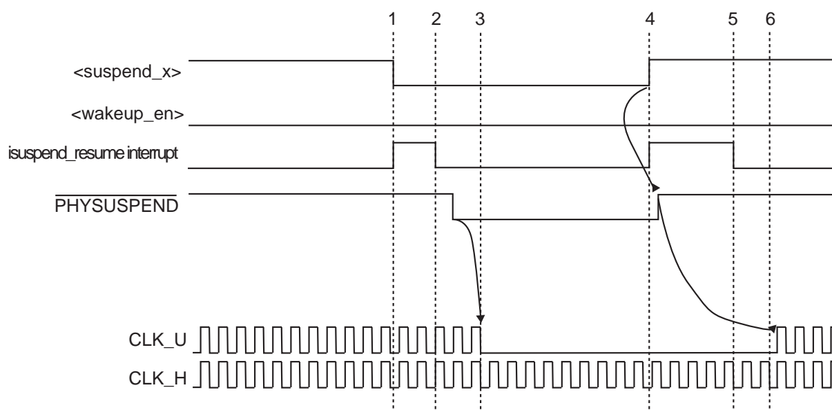
Figure 14-15 Operation of suspend/resume signals (when CLK_H is operating)
