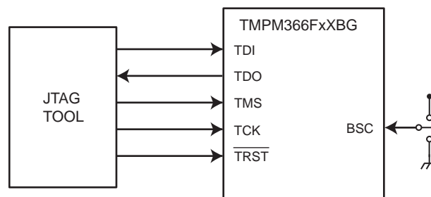
Figure 4-1 Example of connection with a JTAG development tool
