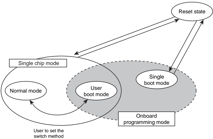
Figure 20-2 Mode Transition Diagram
