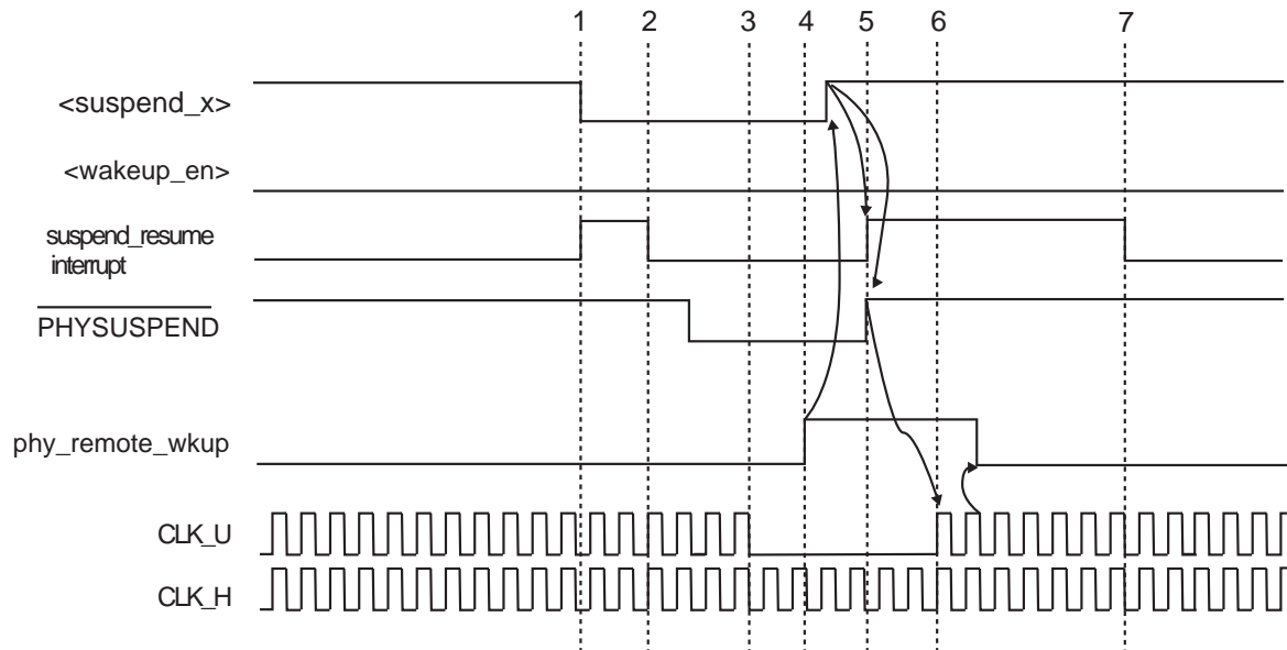
Figure 14-16 Operation of suspend/remote wakeup signals
