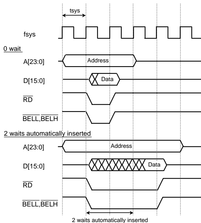
Figure 12-5 Read Operation Timing
