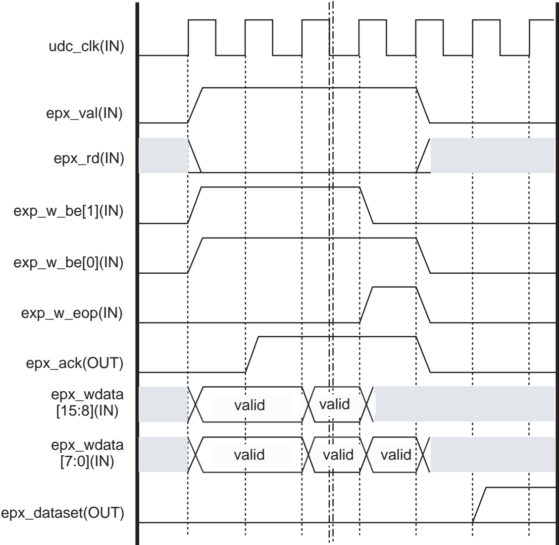
Figure 14-29 MPS (odd number) write access with max_pkt = even number (EP direct access)
