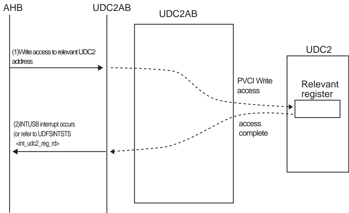
Figure 14-8 Write access for UDC2 register
