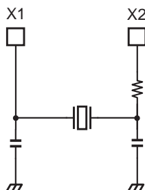
Figure 23-2 High-frequency oscillation connection
