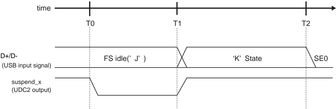
Figure 14-26 Resume operation timing by the host
