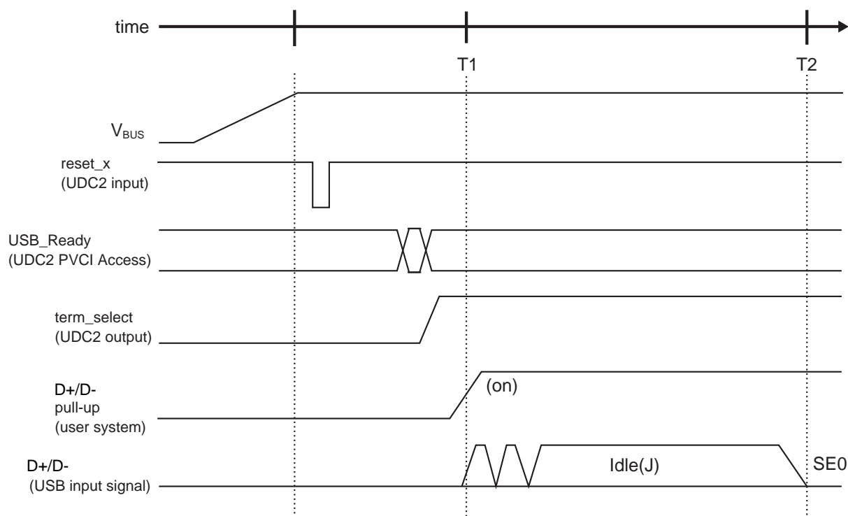
Figure 14-23 Connect operation timing
