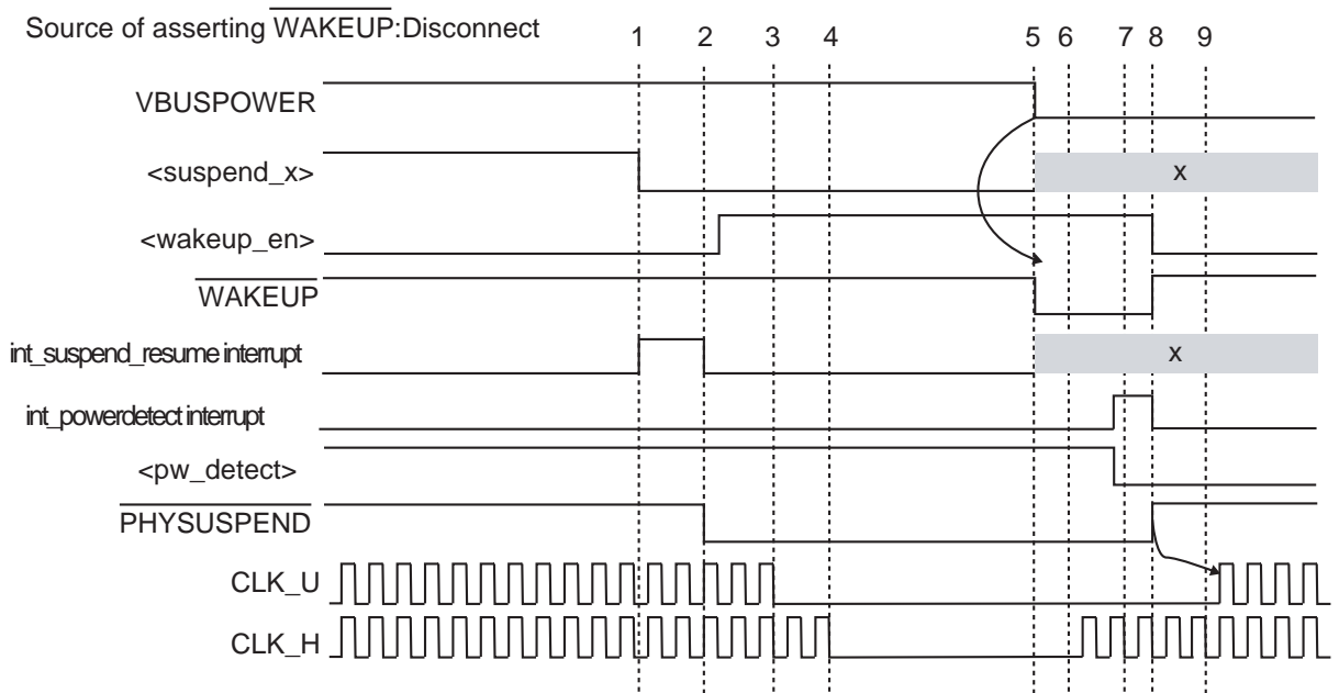
Figure 14-14 Operation of suspend/disconnect signals (when CLK_H is stopped)
