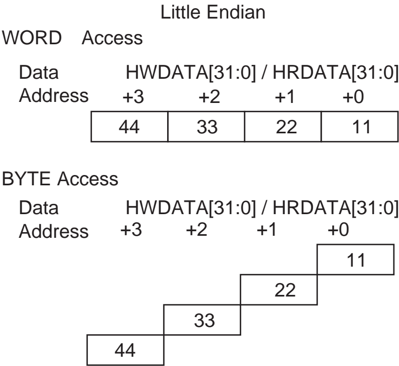
Figure 14-3 Image of Endian conversion in AHB Master function
