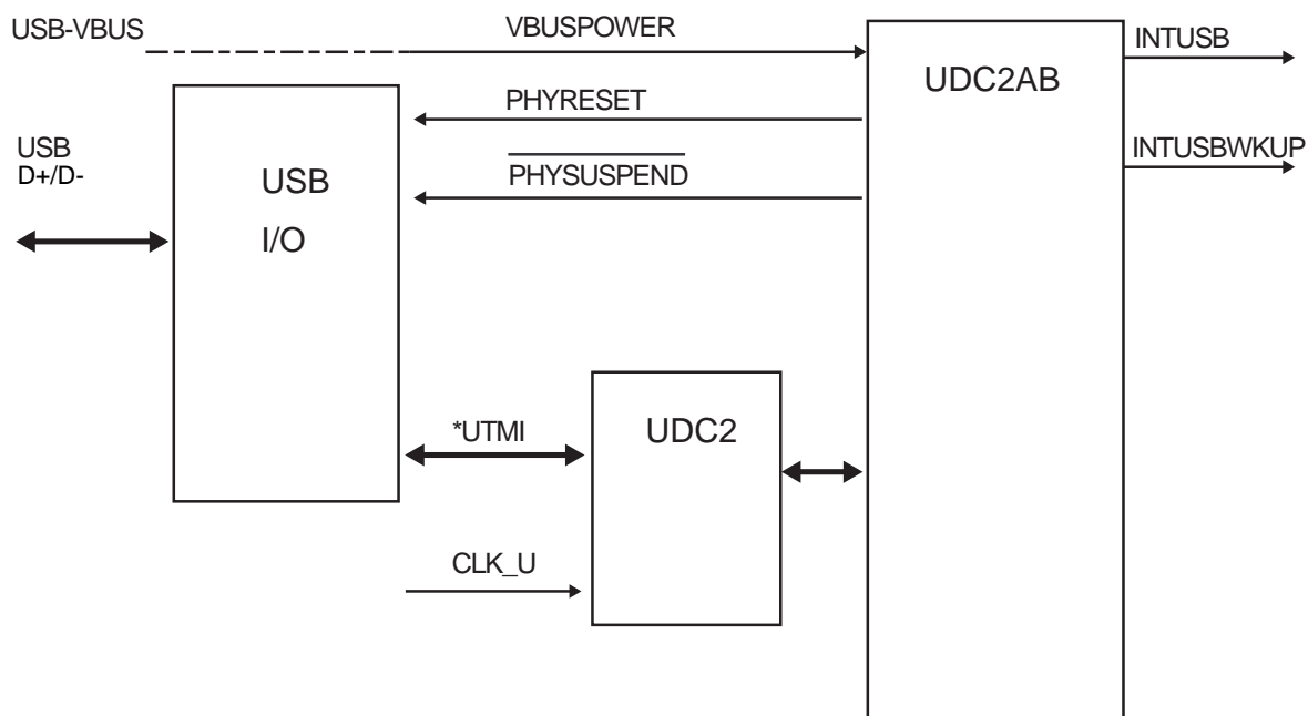
Figure 14-12 Connection diagram of control signals
