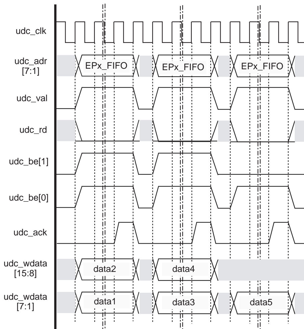
Figure 14-28 MPS write access with max_pkt = odd number (common bus access)
