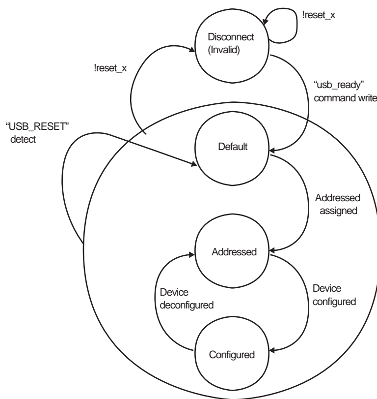
Figure 14-18 Device state diagram
