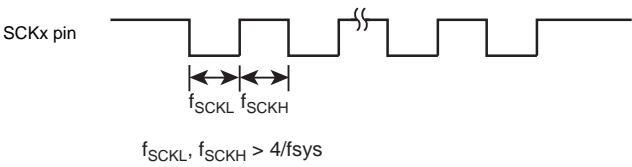
Figure 18-16 Maximum Transfer Frequency of External Clock Input
