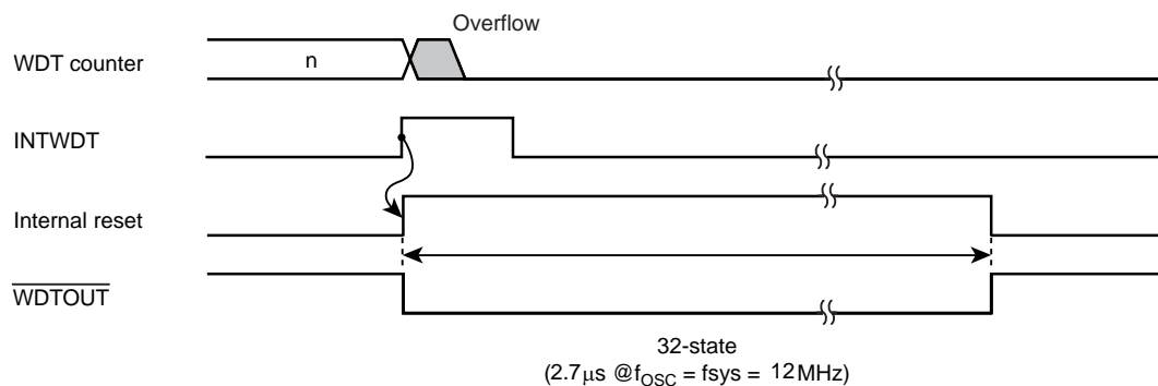
Figure 7-3 Internal reset generation
