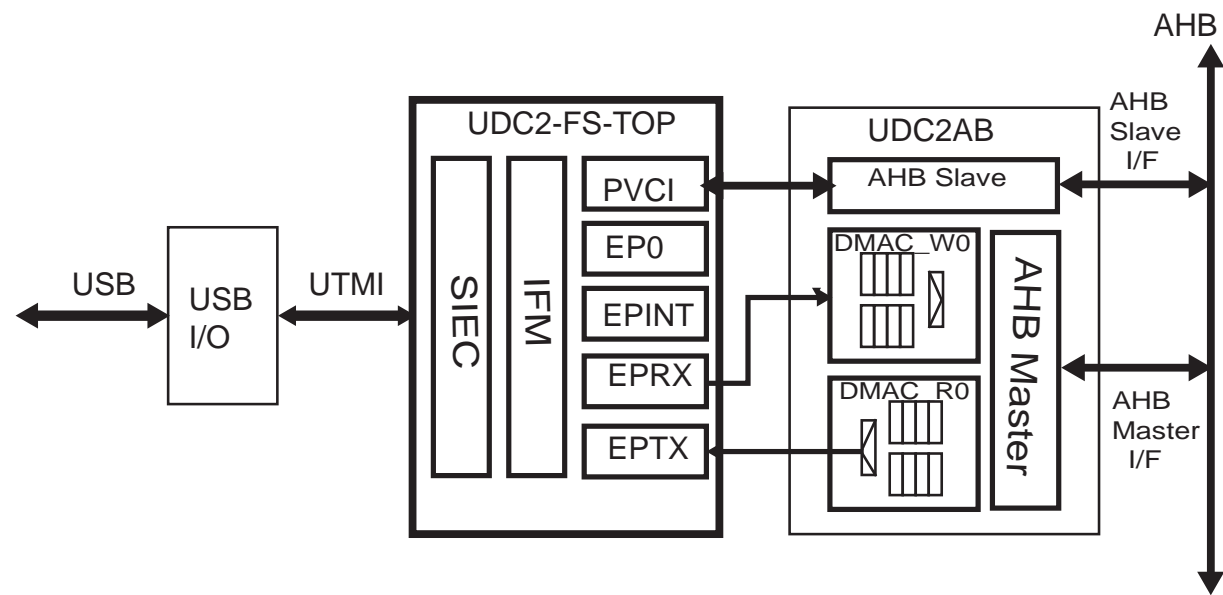
Figure 14-17 Block diagram of UDC2
