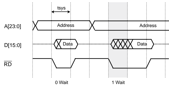
Figure 12-3 Read Operation Timing (0 Wait and 1 Wait Automatically Inserted)
