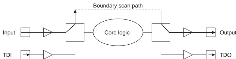
Figure 4-7 Test Data Flow when the EXTEST Instruction is Selected
