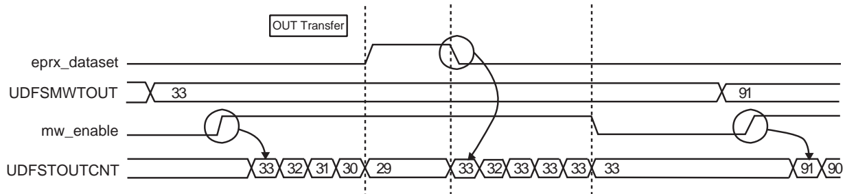
Figure 14-11 Example of MW timeout count
