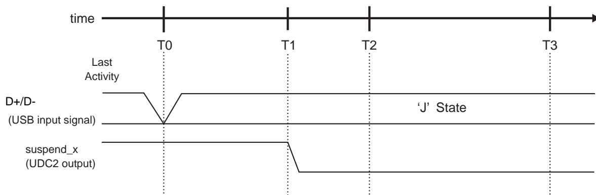
Figure 14-25 Suspend operation timing in FS mode
