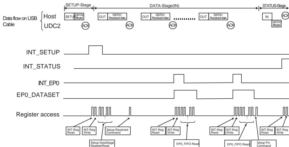
Figure 14-21 Flow of control in Control-WR transfers(with DATA-Stage)
