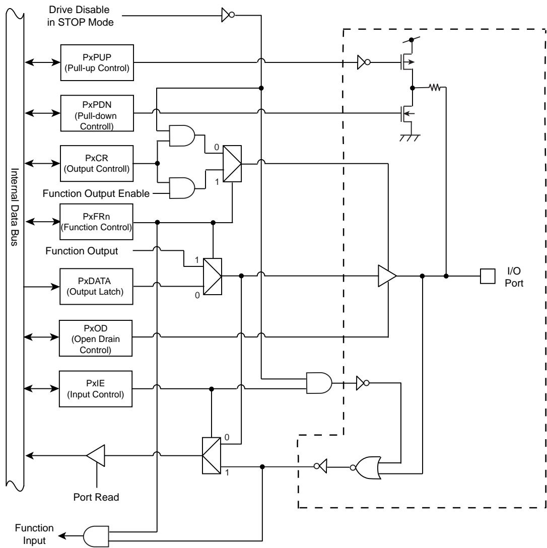
Figure 10-2 Port type FT2
