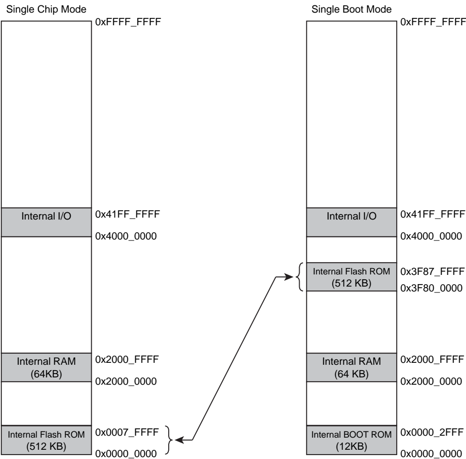
Figure 20-3 Memory Maps for TMPM366FDXBG/FYXBG/FWXBG
