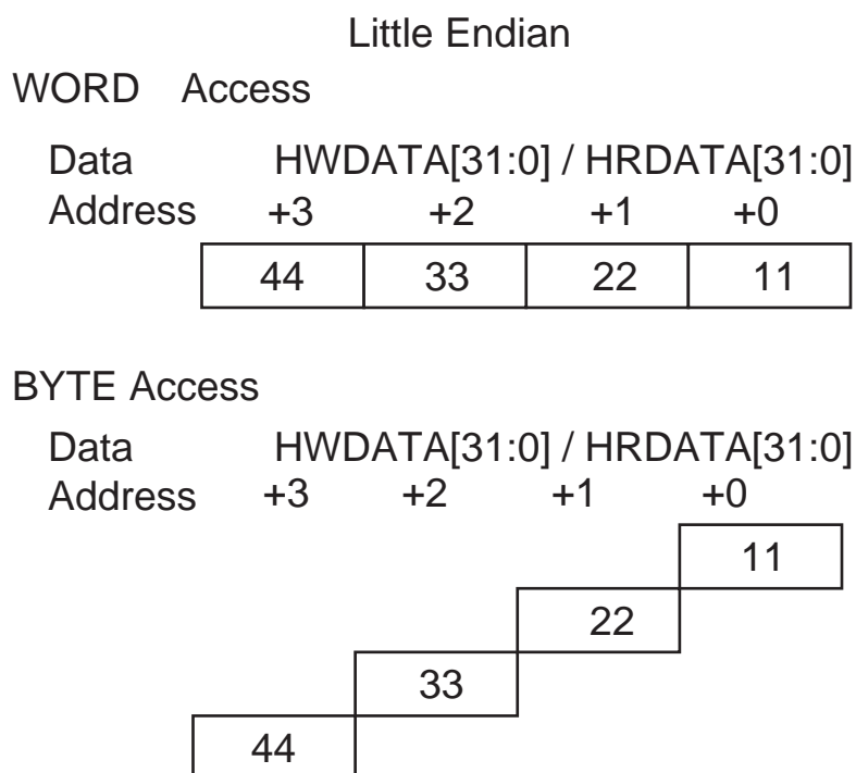
Figure 14-4 Image of Endian conversion in AHB Slave function
