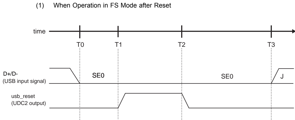
Figure 14-24 Reset operation timing (FS mode)
