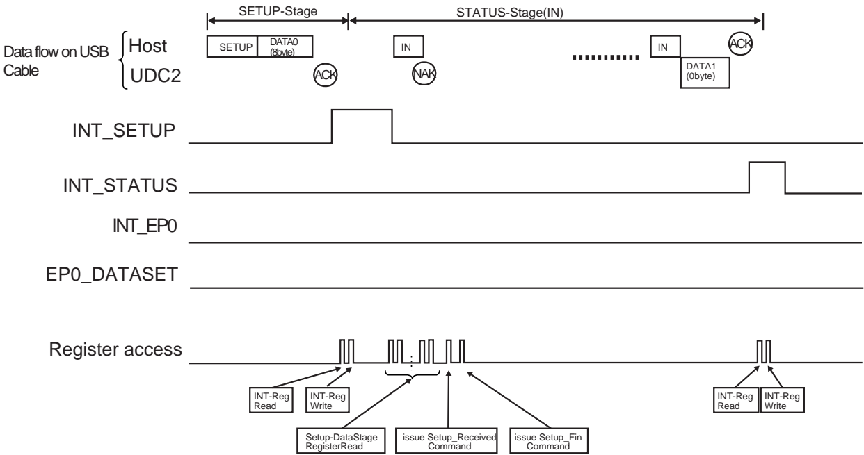
Figure 14-20 Flow of control in Control-WR transfer (without DATA-Stage)
