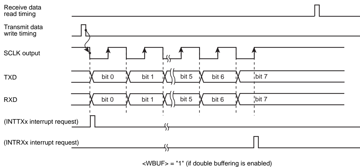
Figure 15-16 Transmit/Receive Operation in the I/O Interface Mode (SCLK Output Mode)
