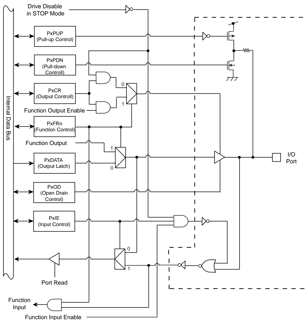
Figure 10-7 Port Type FT7
