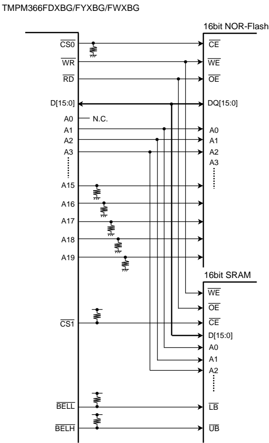
Figure 12-19 Connection Example for external 16-bit SRAM and NOR-Flash
