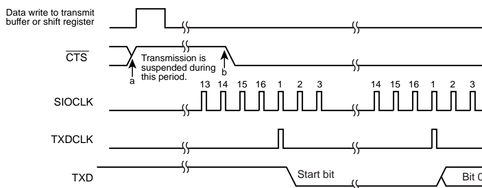
Figure 15-9 \overline{\text{CTS}} Signal timing
