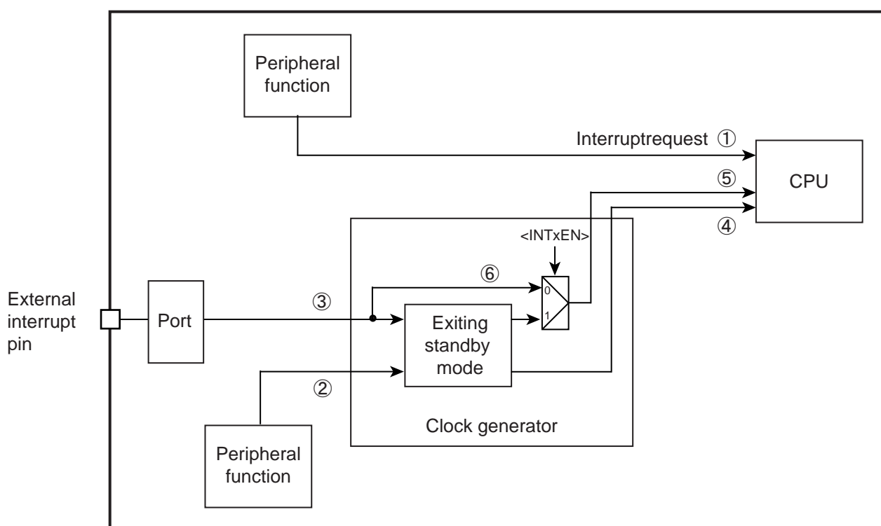
Figure 9-1 Interrupt Route
