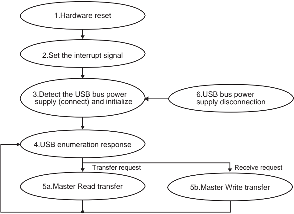
Figure 14-10 Overall operation sequence
