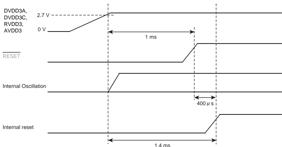
Figure 6-1 Cold Reset Sequence
