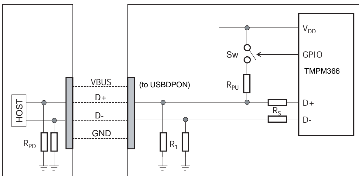
Figure 23-1 Example Circuit
