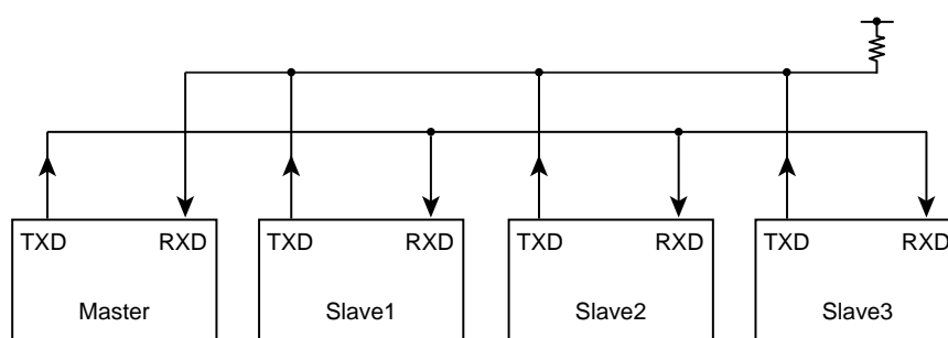
Figure 15-18 Serial Links to Use Wake-up Function
