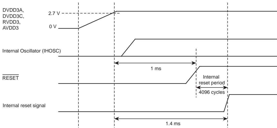
Figure 23-3 Power-on sequence
