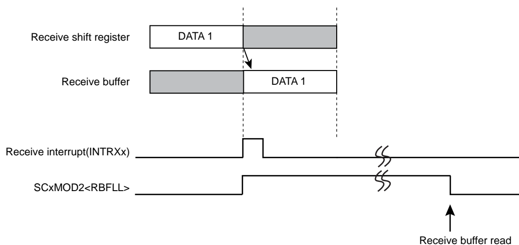
Figure 15-4 Receive Buffer Operation
