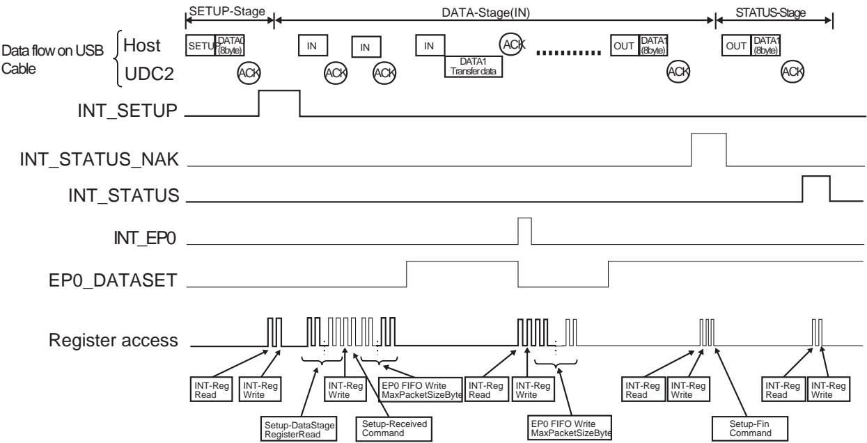
Figure 14-22 Example of using the INT_STATUS_NAK flag in Control-RD transfers
