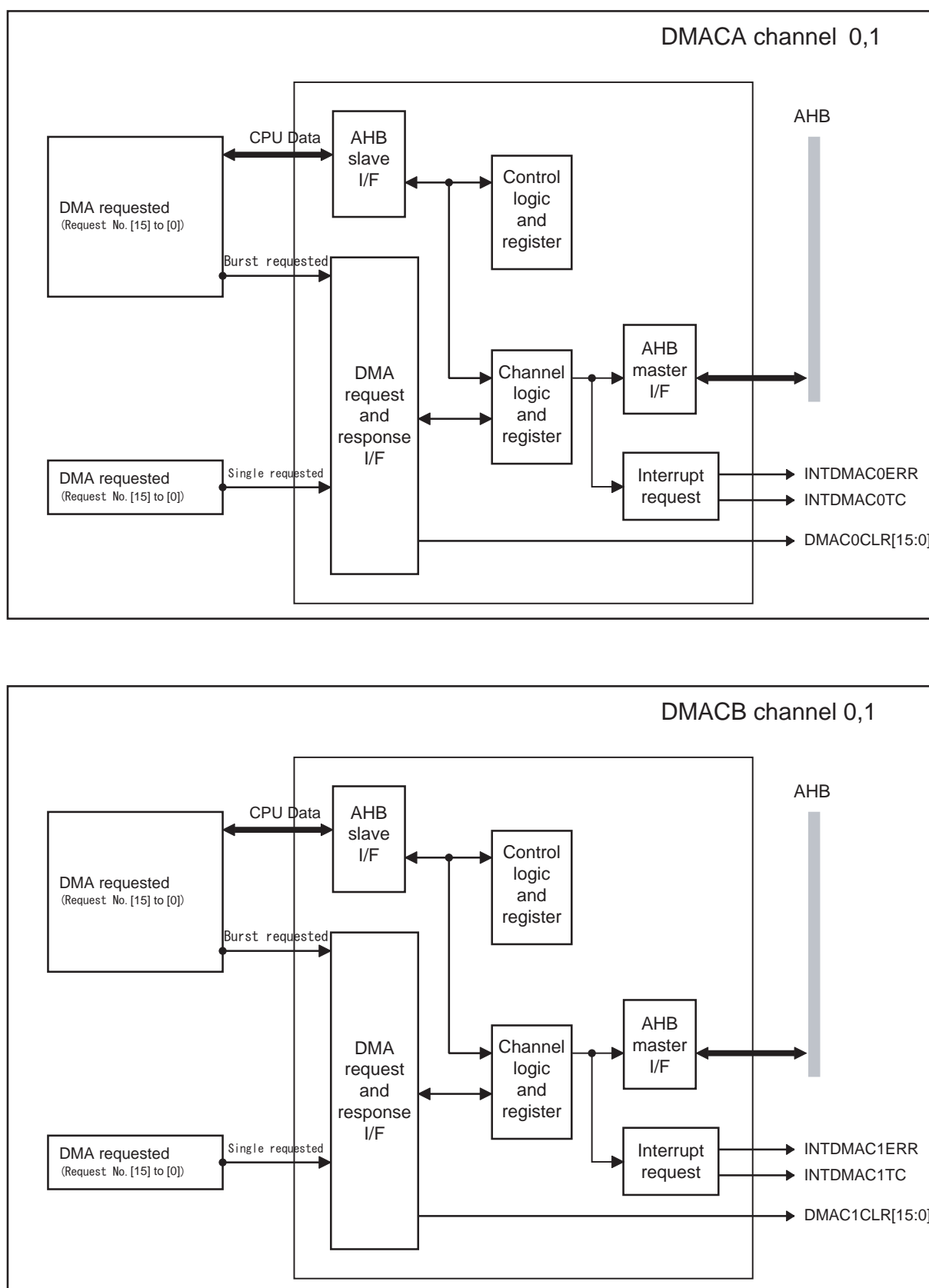
Figure 11-1 DMAC Block diagram
