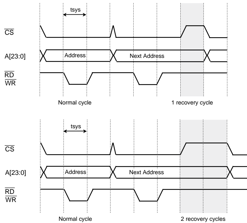
Figure 12-8 Timing of Chip Select Recovery Time Insertion
