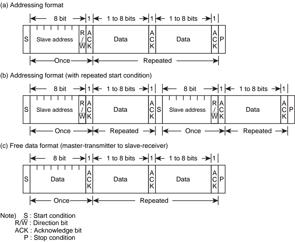
Figure 18-2 I2C Bus Mode Data Formats
