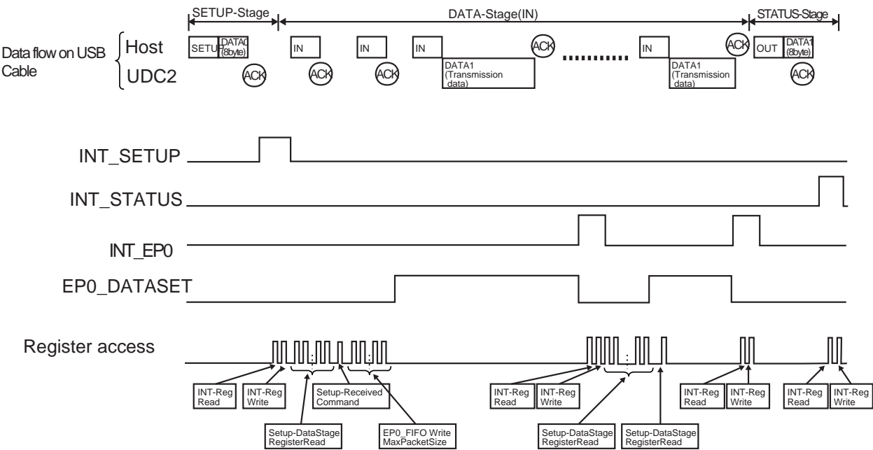
Figure 14-19 Flow of the control in Control-RD transfer
