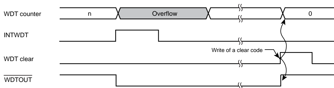
Figure 7-2 INTWDT interrupt generation
