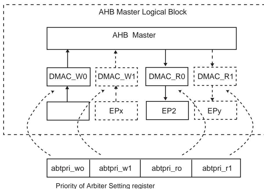
Figure 14-6 Relationship between DMAC and priority areas
