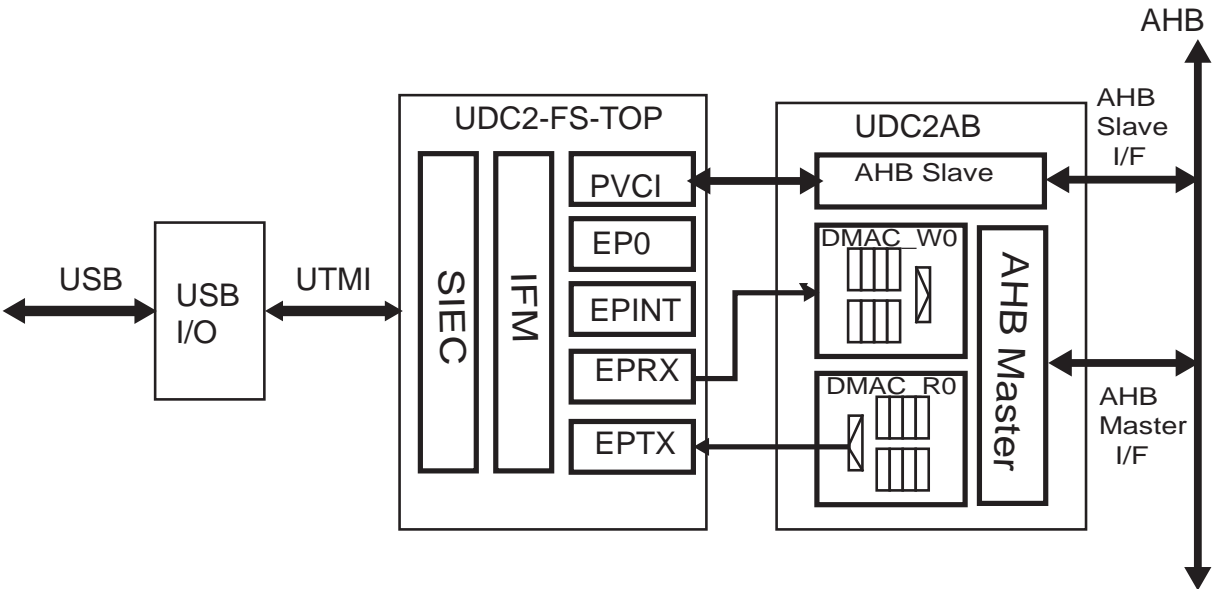
Figure 14-1 Block diagram of the USB device controller
