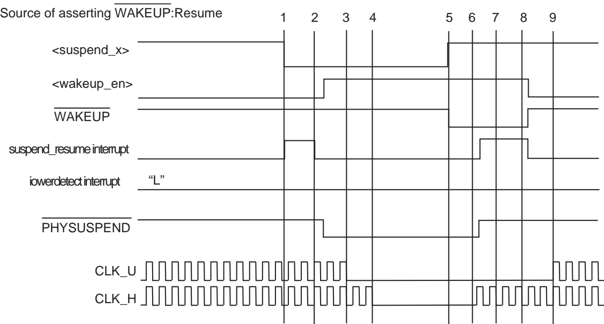
Figure 14-13 Operation of suspend/resume signals (when CLK_H is stopped)
