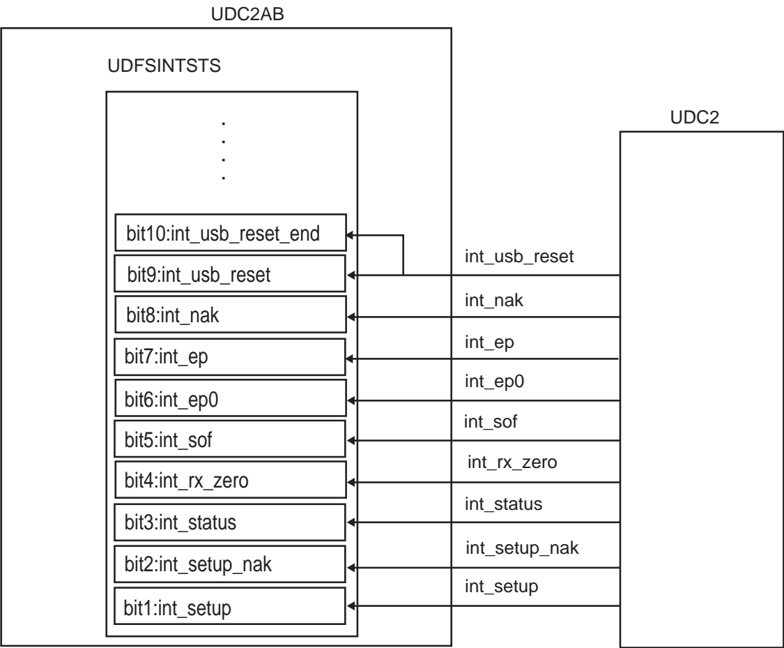
Figure 14-5 Connection between the flag output signals and interrupt bits.
