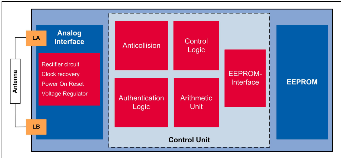
Figure 6 Block Diagram
