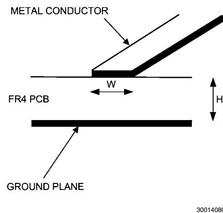
FIGURE 15. Microstrip Configuration
