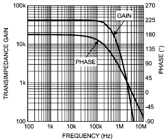
Output Amplifier Gain & Phase vs. Frequency
