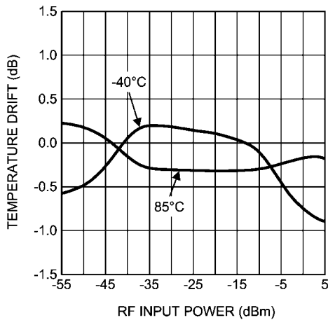
Mean Temperature Drift Error vs. RF Input Power at 50 MHz
