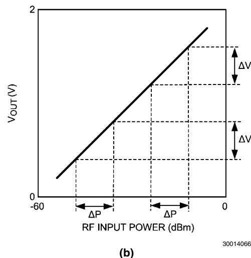
FIGURE 1. Convex Detector Transfer Function (a) and Linear Transfer Function (b)
