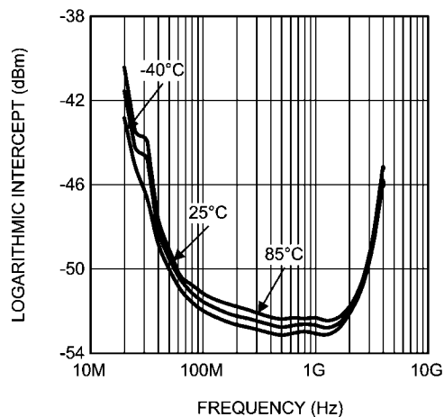
Log Intercept vs. Frequency
