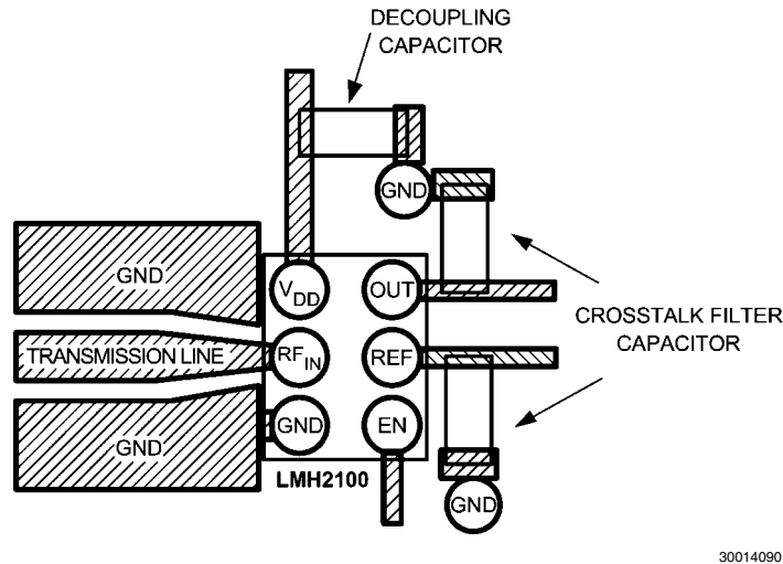
FIGURE 14. Recommended Board Layout
