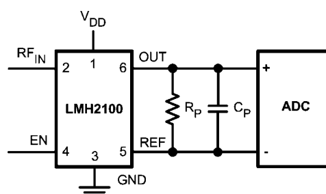
FIGURE 12. Single Ended and Differential Application
