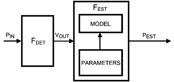
FIGURE 5. Generic Concept of a Power Measurement System
