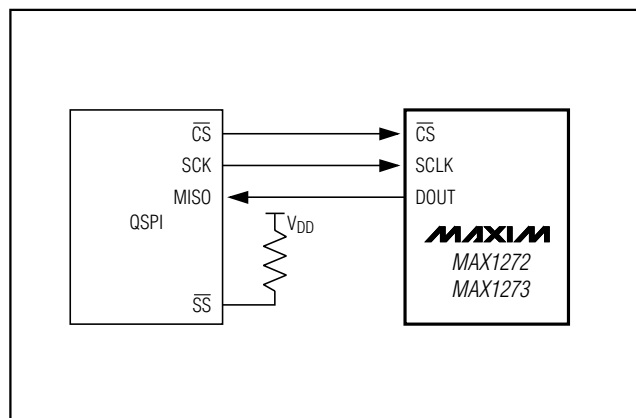
Figure 11. QSPI Connections
