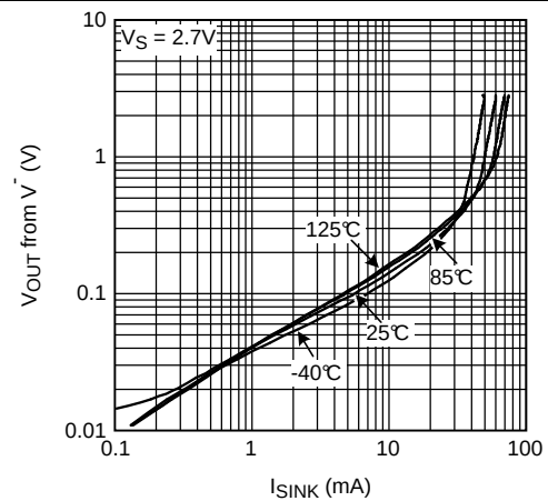
Figure 2. Output Swing vs. Sinking Current
