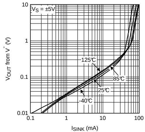
Figure 4. Output Swing vs. Sinking Current
