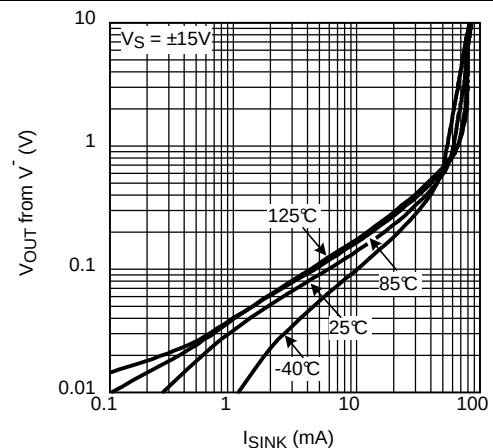
Figure 6. Output Swing vs. Sinking Current
