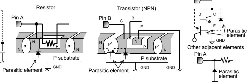
Fig.28 Simplified structure of monoristic IC
