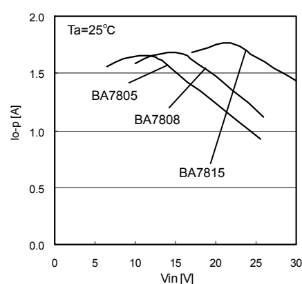
Fig.18 Peak Output Current
