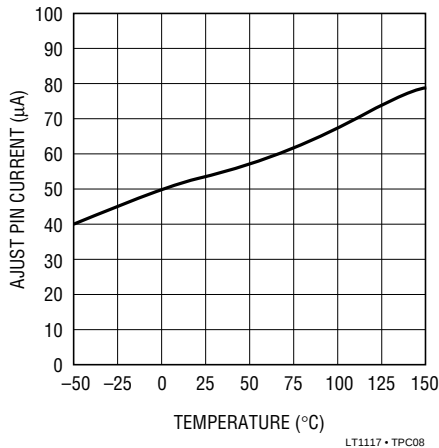
Adjust Pin Current
