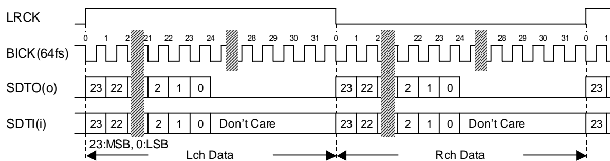
Figure 4. Mode 2/6 Timing
