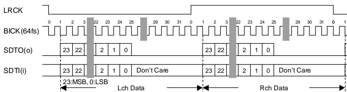
Figure 5. Mode 3/7 Timing
