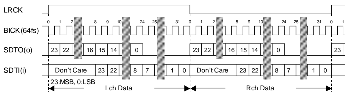
Figure 3. Mode 1/5 Timing
