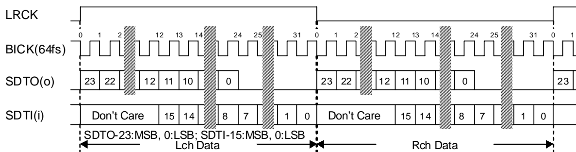
Figure 2. Mode 0/4 Timing
