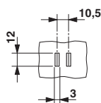
Dimensional drawing
