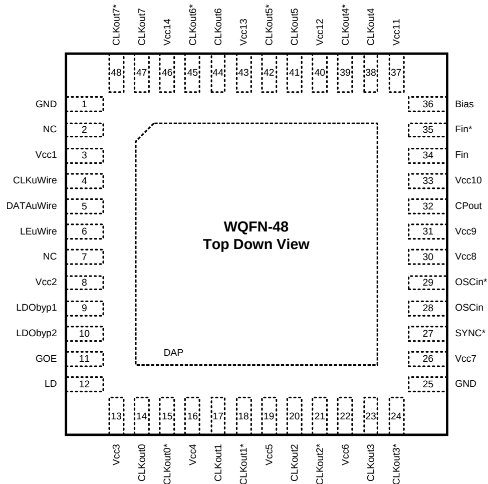
Pin Descriptions
