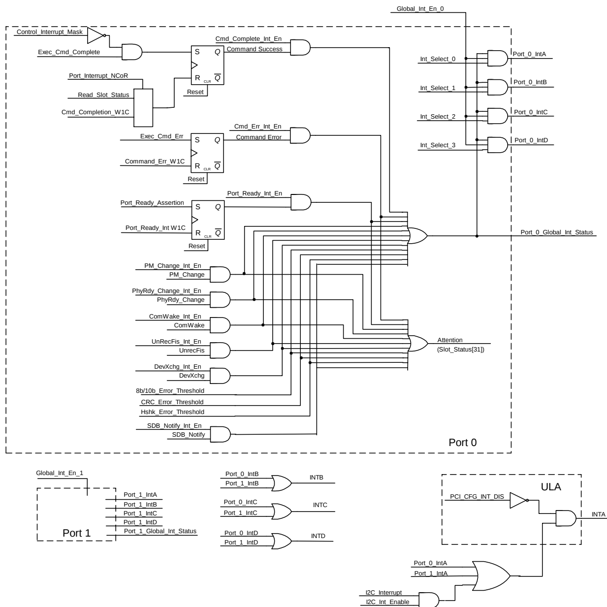
Figure 5-3 Sil3531A Interrupt Map
