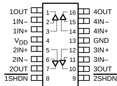
TLV2785 D, N, OR PW PACKAGE (TOP VIEW)
