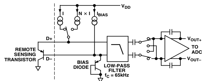
Figure 3. Signal Conditioning
