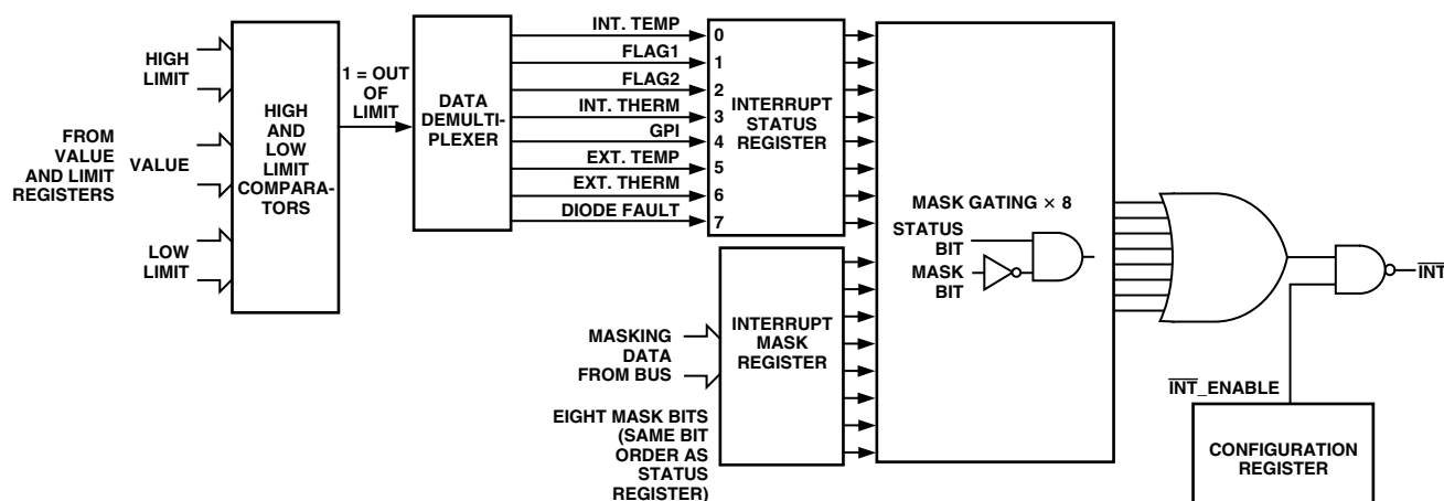
Figure 9. Interrupt Register Structure
