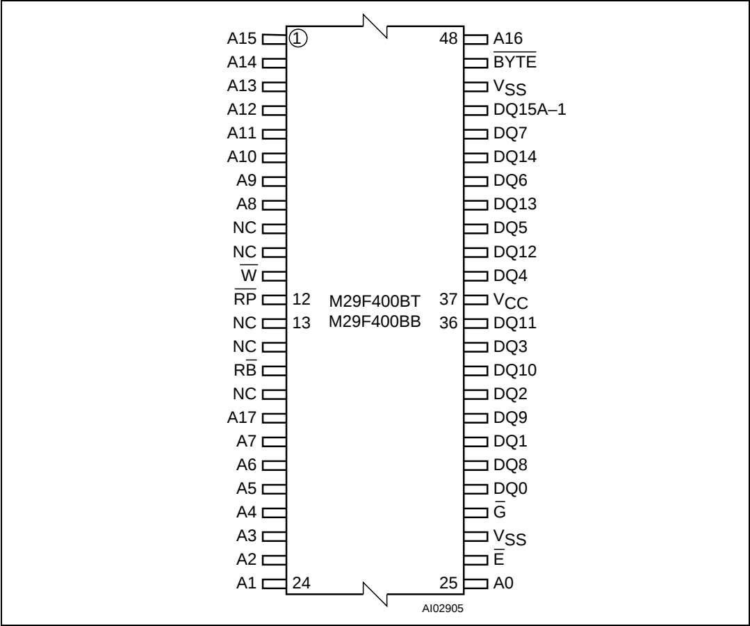
Figure 2. TSOP connections
