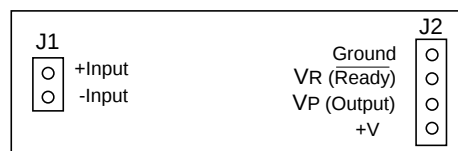
EH300/EH301 Top View
