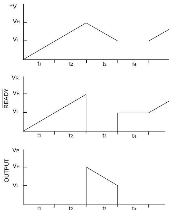
EH300/EH301 Waveforms
