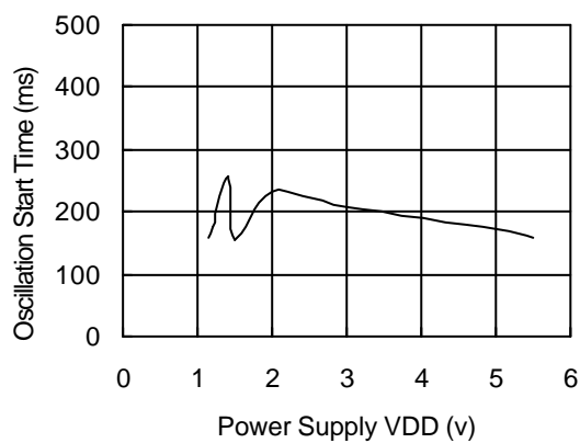
Oscillation Start Time vs. Power Supply (T opt =25°C)
