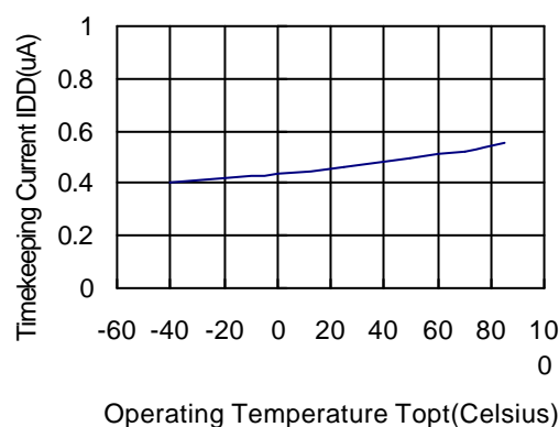
Timekeeping current vs. Operating Temperature (with no 32-kHz output) (Output=Open, V_{DD}=3\text{V} )
