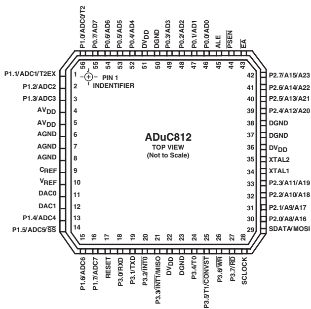
56-Lead LFCSP
