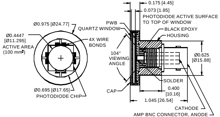
BNC CONNECTOR PACKAGE ACTIVE AREA = .4447 (11.295) DIA = 100 mm 2
