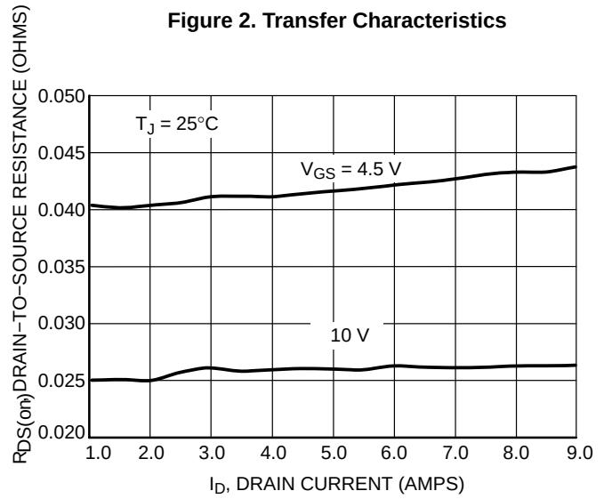
Figure 4. On-Resistance versus Drain Current and Gate Voltage
