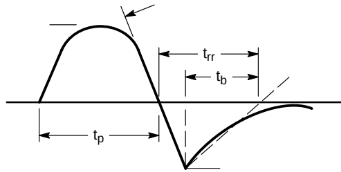
Figure 15. Diode Reverse Recovery Waveform
