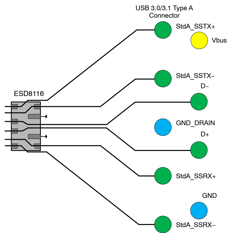
Figure 13. USB 3.0/3.1 Type-A Layout Diagram
