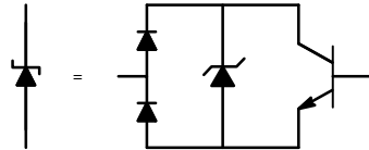
Figure 1. Pin Schematic
