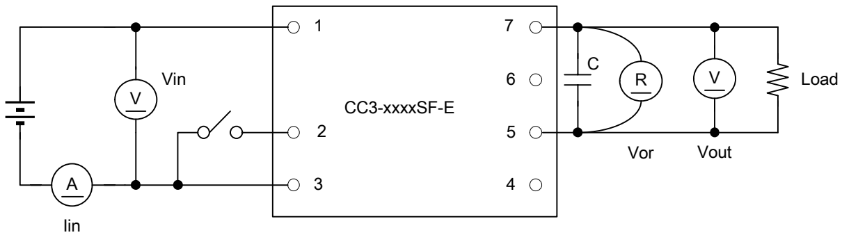
[5] Test Circuit
